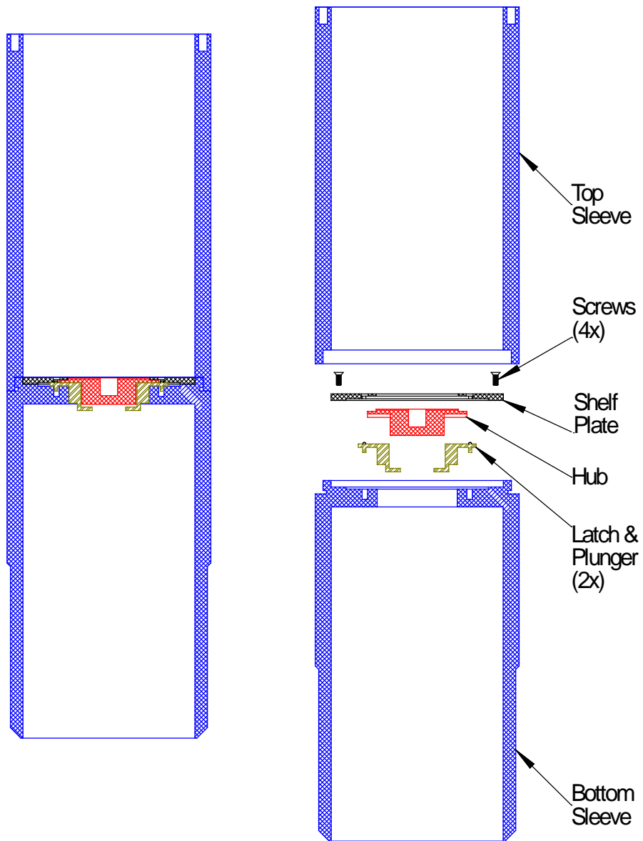
Figure 4 – 3013 Carrier Design
