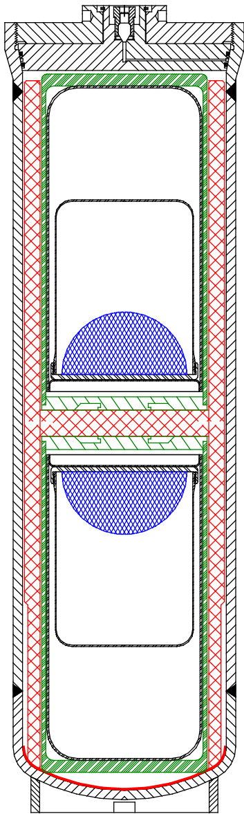
Figure 2 – 3013 Carrier Loading
