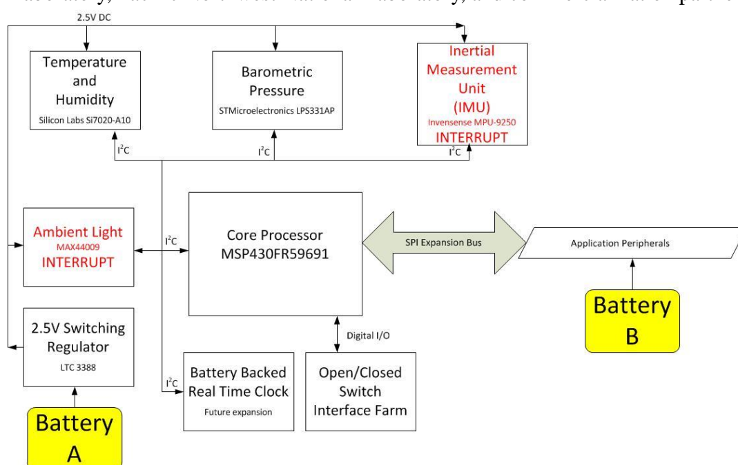
Figure 1. The ACTS Motherboard Architecture, built on the low-power MSP family of processors, incorporates a base set of relevant sensors and a peripheral interface for matching ACTS to specific applications.
