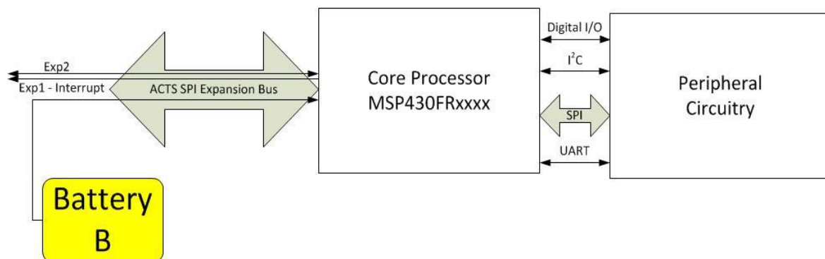
Figure 3. Using a processor in the peripheral reference design allows interfacing flexibility and commonality among the peripherals.
