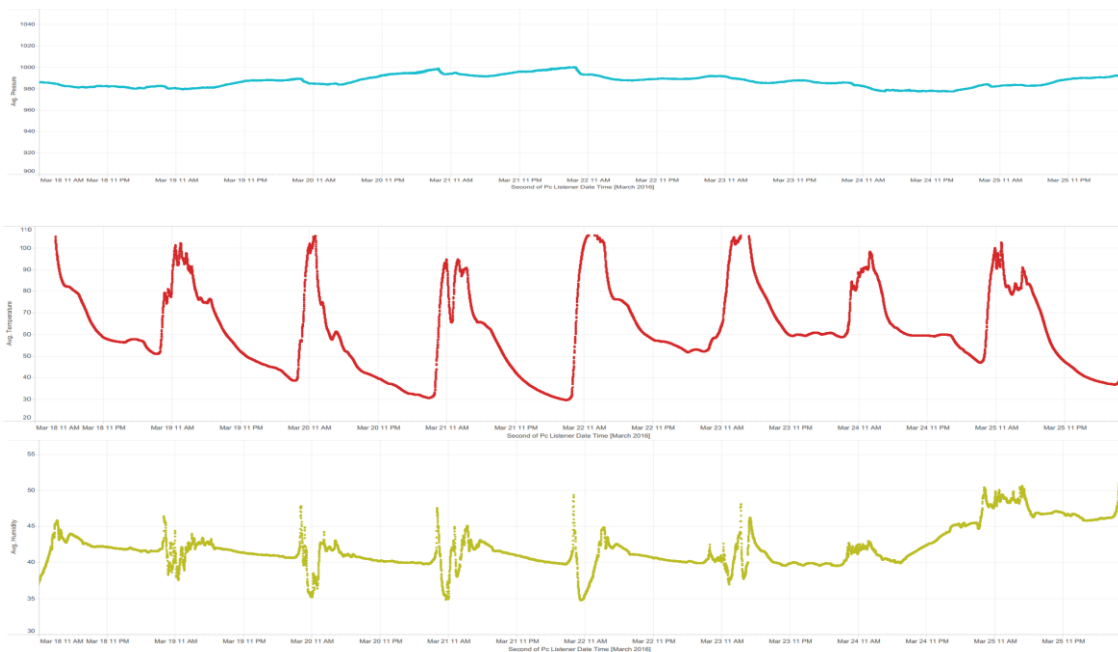
Figure 9. Outdoor barometric pressure, temperature, and relative humidity collection, March 18 to 25, 2016.
