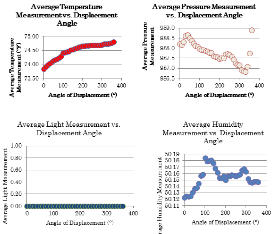
Figure 12. Example environmental sensor measurement.
