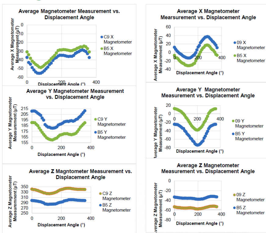
Figure 11. Typical magnetometer results.
