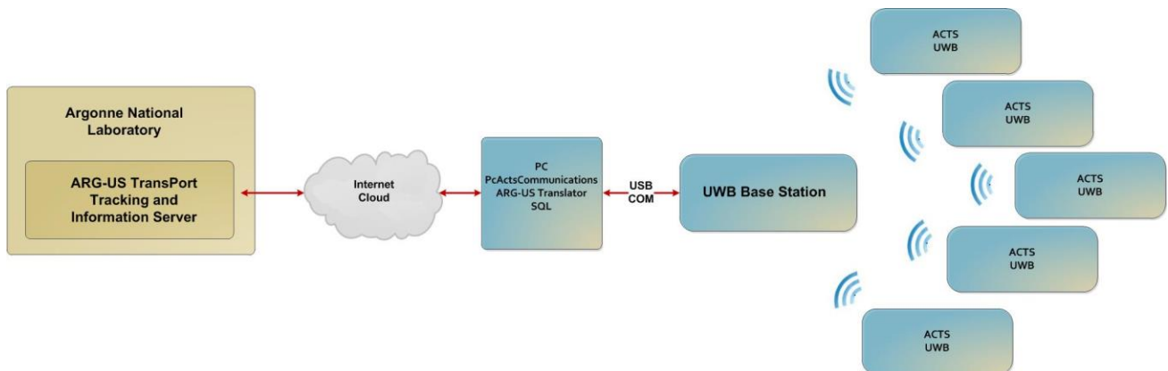
Figure 4. The testing hardware configuration used five different tags and various servers that collected ACTS messages.
