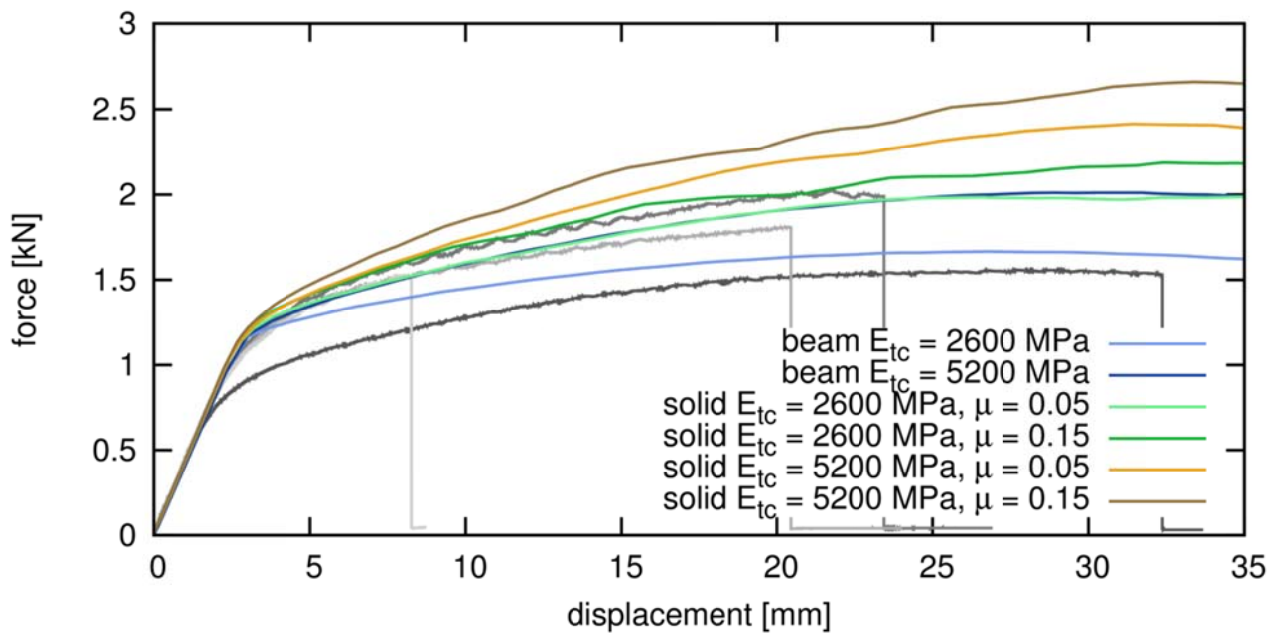
Figure 5 Results of solid element calculation in comparison with beam calculation
