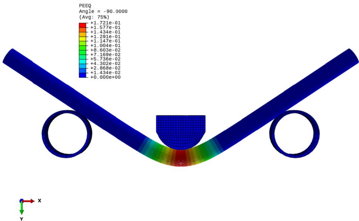
Figure 2 Finite element model of 3-point bending test with beam elements: plastic strains in the last calculation step
