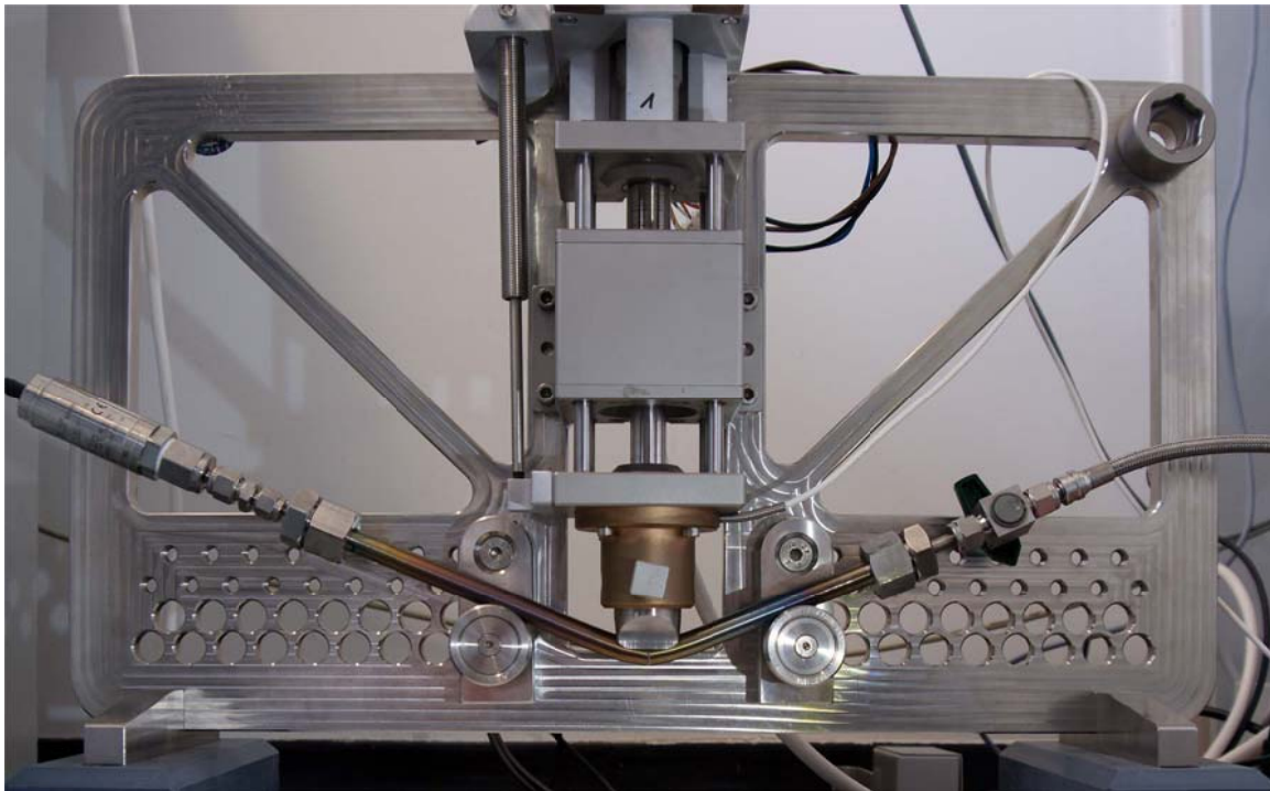
Figure 1 Test setup for quasi-static 3-point bending test
