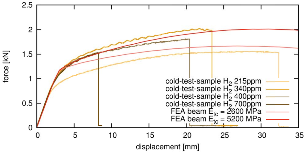
Figure 3 Results of beam element calculation in comparison with cold test results
