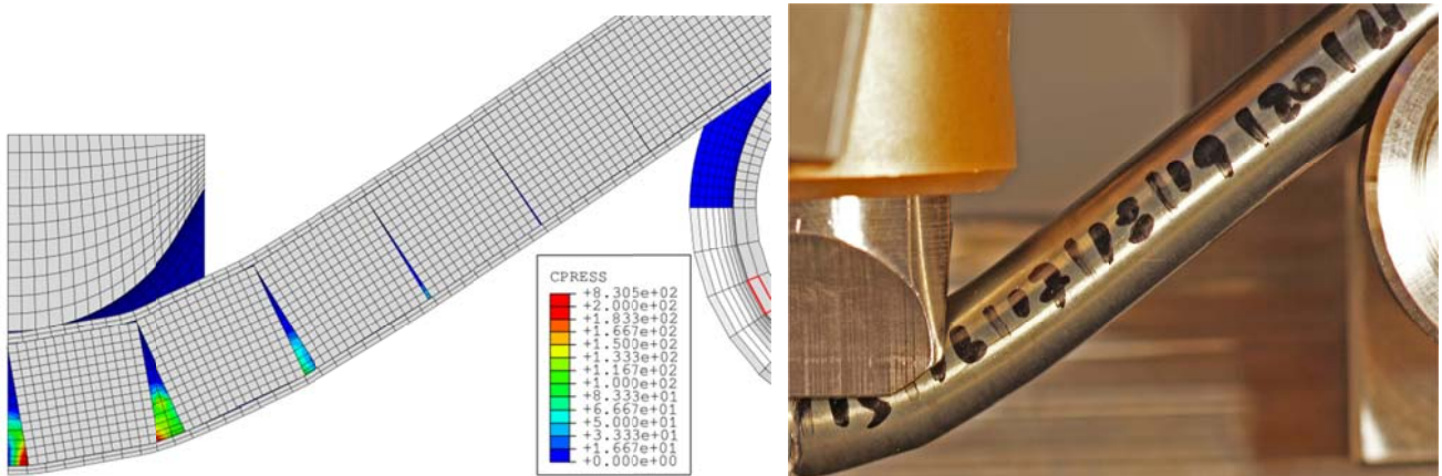
Figure 4 Finite element model of 3-point bending test with solids elements: contact pressure in the last calculation step in comparison with experimental results
