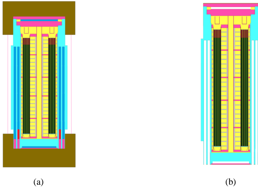
Figure 5. Cross sections of the computational model of TUK-153 with SNF for dose rates calculation: under normal conditions – (a); b - under accident conditions – (b) All simplifications of the actual packaging design, such as construction tolerances as well as the absence of some structural elements and freight pins, are conservative and lead to an overestimation of dose rate beyond the TUK-153 protection.
