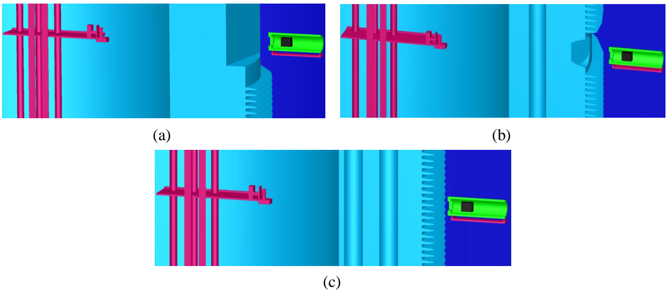
Figure 10. Locations of the detector number 1 – (a), number 2 – (b) and number 3 – (c) in computational model
