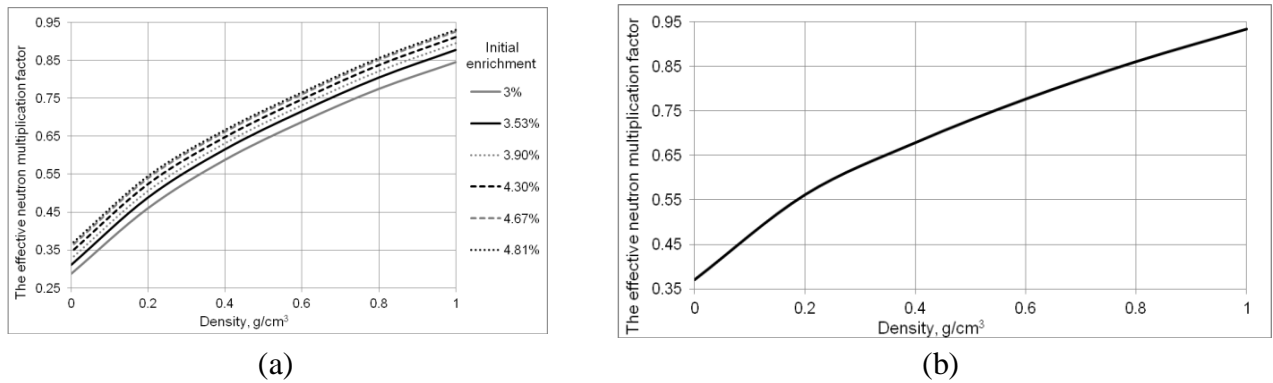
Figure 2. Dependence of K_{eff} on the steam-water mixture density in the TUK-153 for a single package (depends on ^{235}\text{U} initial enrichment) – (a) and for an infinite number of packages ( ^{235}\text{U} initial enrichment 4,925 %) – (b)
