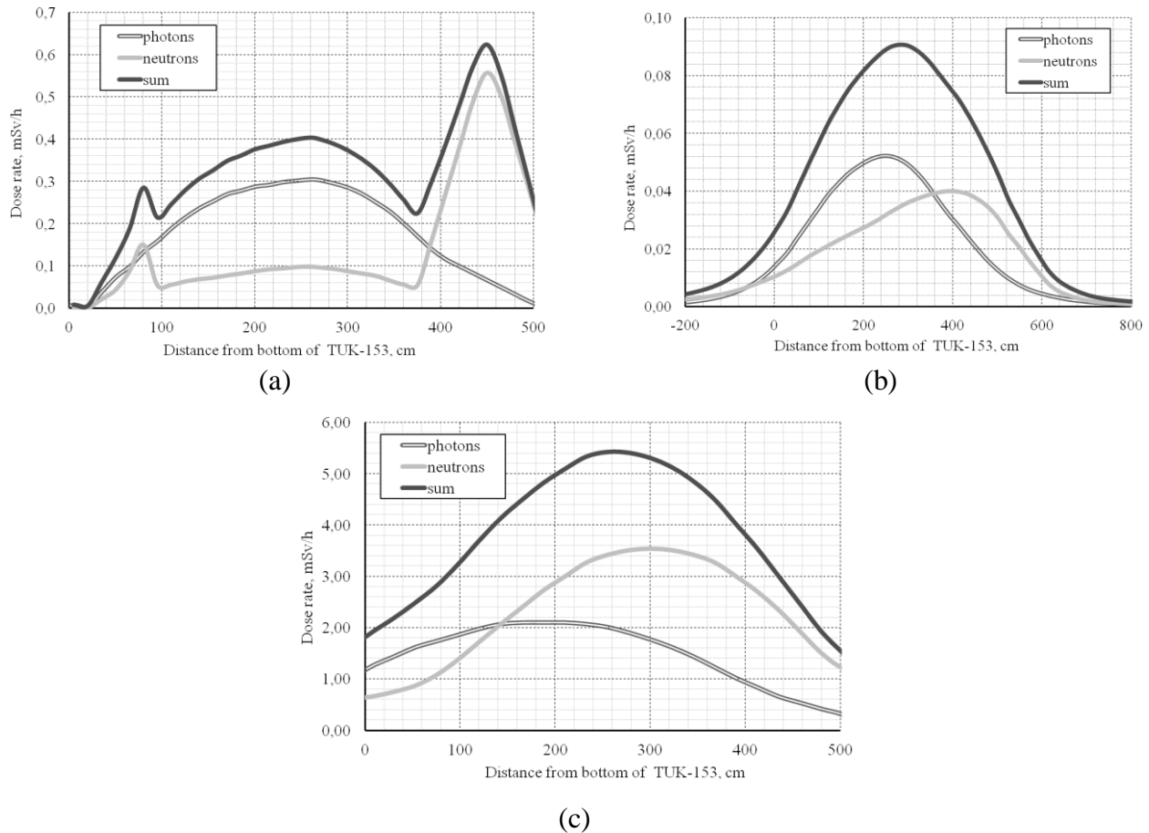
Figure 6. The distribution of dose rate at the surface of TUK-153 under normal conditions – (a), at 2 m from the surface of TUK-153 under normal conditions – (b), at 1 m from the surface of TUK-153 under accident conditions – (c)
