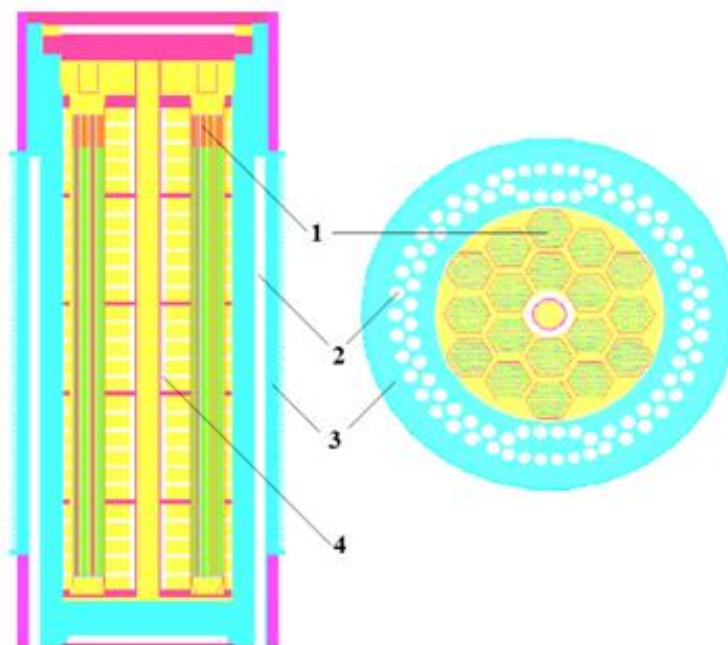
Figure 1. Cross sections of the computational model of TUK-153 with SNF for K_{eff} calculation in normal conditions of transport
