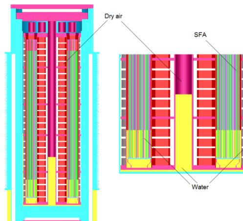
Figure 3. Cross section of the computational model of TUK-153 with SNF
