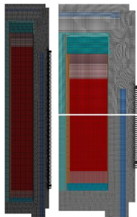
Figure 13. Two-dimensional axial-symmetric computational model of TUK-153
