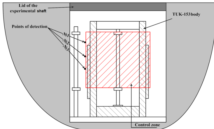
Figure 8. Scheme of experimental stand
