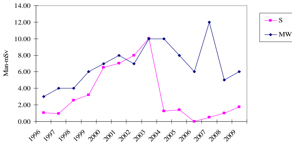
Figure 1. Collective dose (S) vs. number of monitored workers (MW) by year
