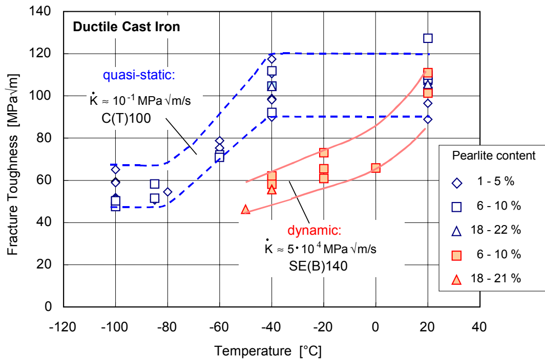
Fig. 2. Influence of loading rate, test temperature and pearlite content on the fracture toughness behaviour of ductile cast iron according to [13, 14]
