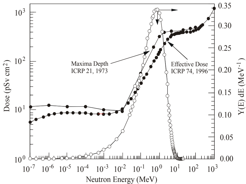
Fig. 1. The maxima neutron dose to fluence conversion of ICRP Publication 21 (1973), which was used in the 1996 edition of the Q-System, and the effective dose to fluence conversion from ICRP Publication 74 (1996.) The Publication 21 data are for normally incident neutrons on a cylindrical phantom, and Publication 74 data are for a rotational exposure geometry of an anthropomorphic phantom. The normalized distribution in energy of neutrons emitted by ^{252}\text{Cf} (from ENDF/B) is shown by the open circle data points.
