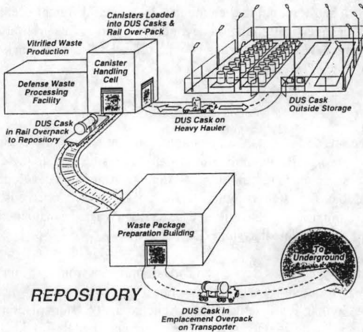
Figure 2. DU-Shielded Cask Scenario
