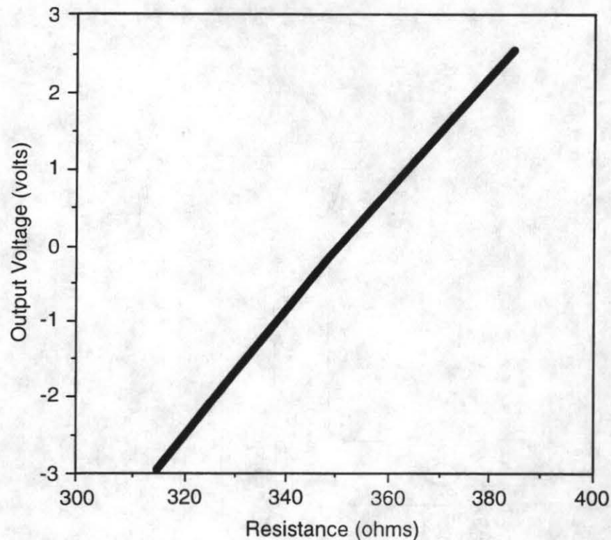
Figure 3. Enhanced strain measurement device output voltage versus resistance change.
