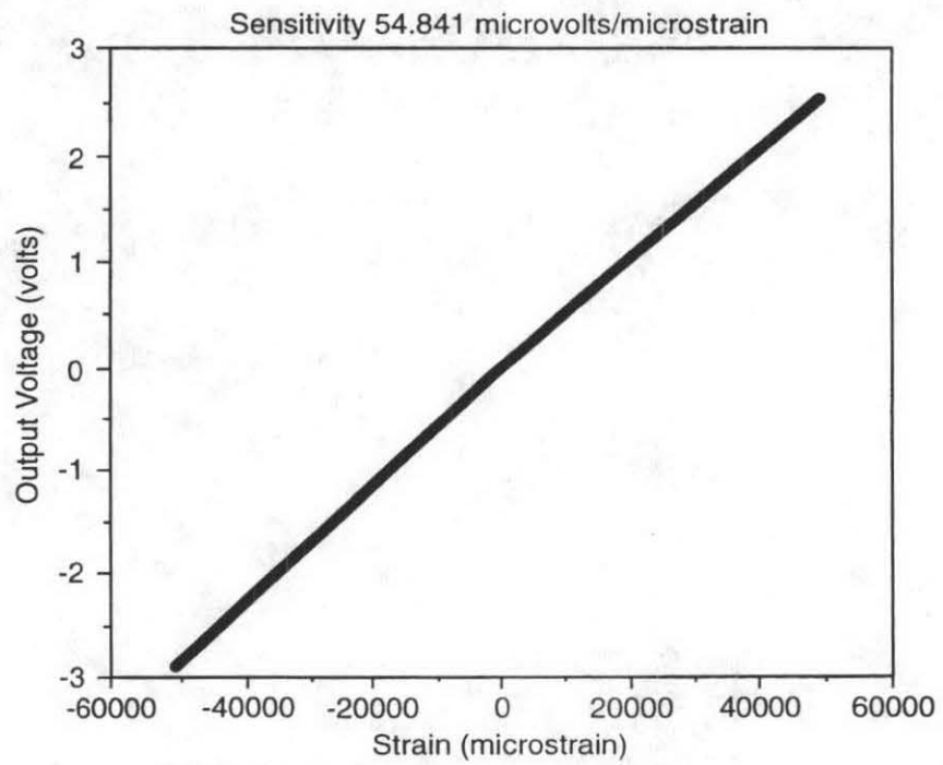
Figure 5. Enhanced strain measurement device sensitivity.
