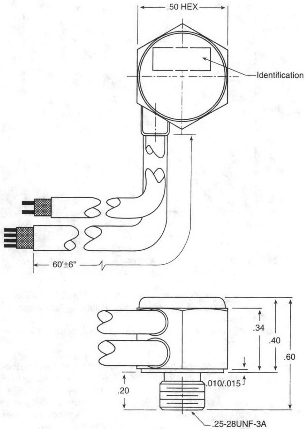
Figure 2. Mechanical configuration of the enhanced strain measurement device. Units in inches.
