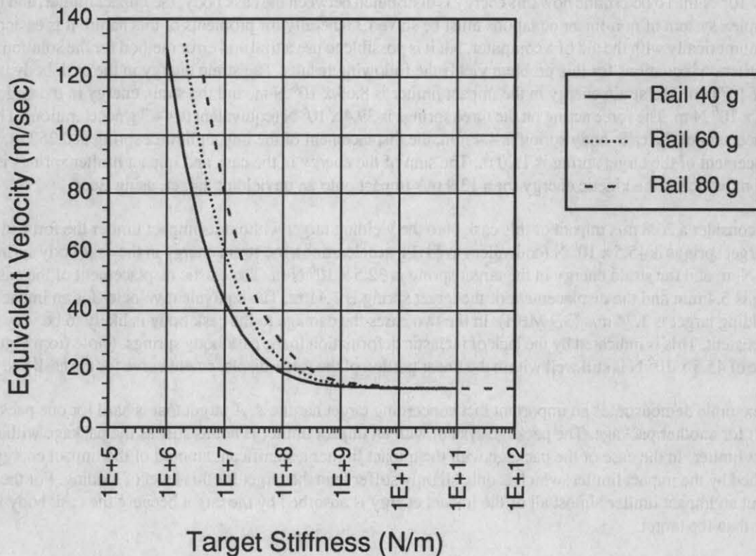
Figure 3 - Impact velocity onto a yielding target that causes the same damage as a 9 m impact onto an unyielding target for a 90,700 kg rail cask.
