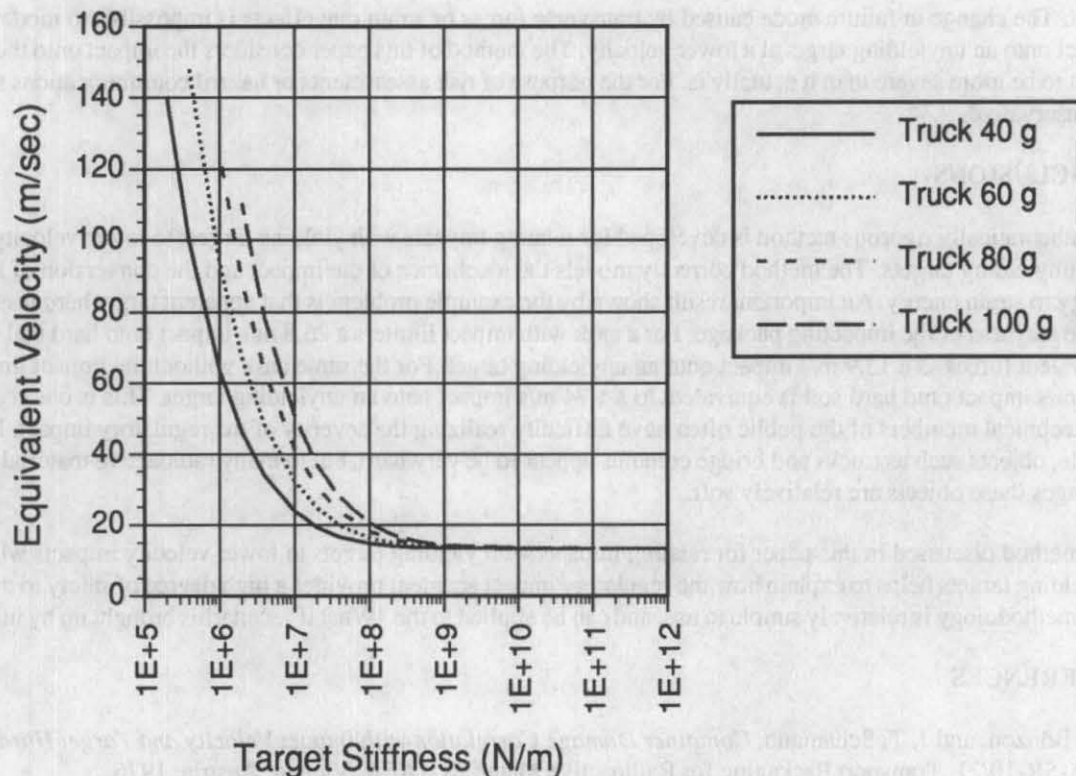
Figure 4 - Impact velocity onto a yielding target that causes the same damage as a 9 m impact onto an unyielding target for a 23,000 kg truck cask.
