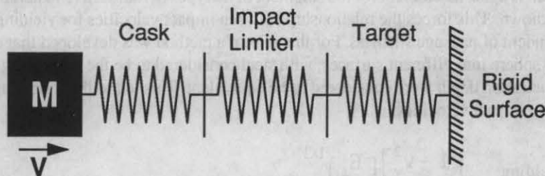
Figure 1 - Simplified spring model for impacts.
