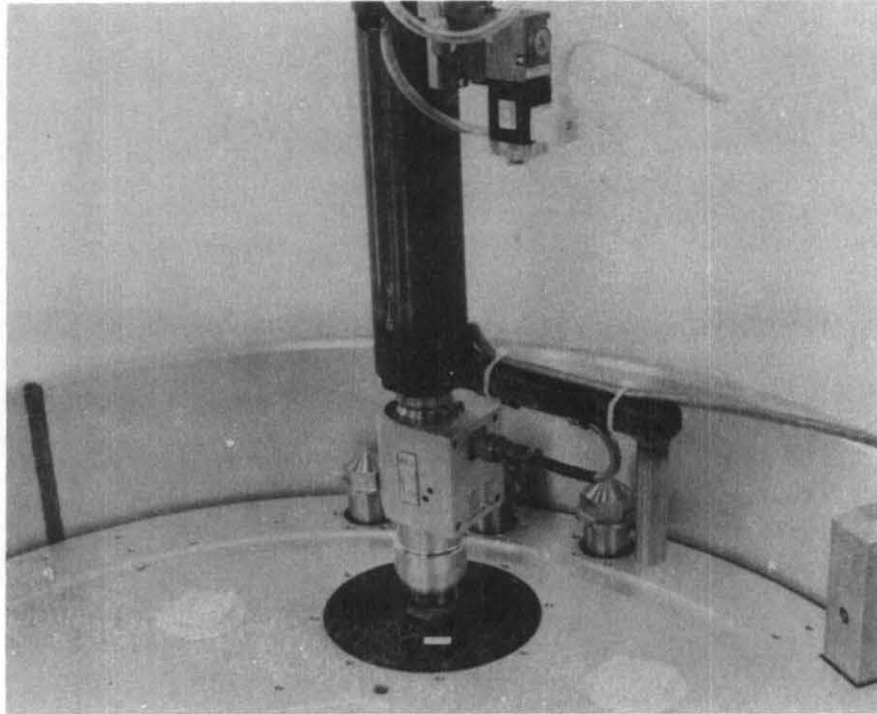
Figure 2: Cask Head Operations (CHO) System
