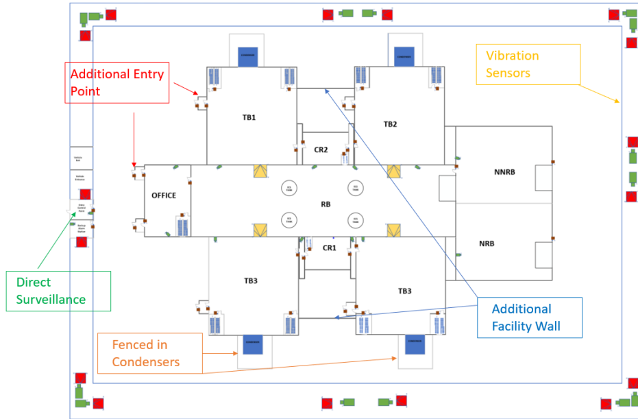
Figure 1. Security-by-Design schematic for a hypothetical SMR, from [5]
