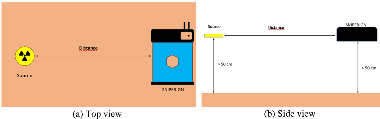
Figure 3: experimental setup
